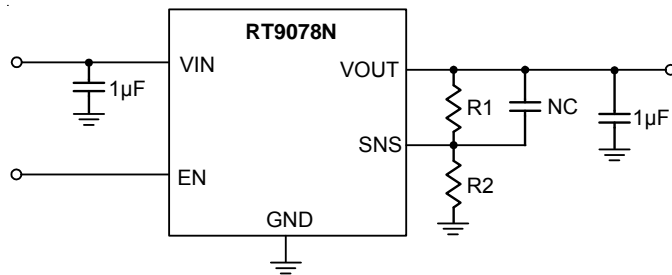
Figure 3. Adjustable Output Voltage Application Circuit
